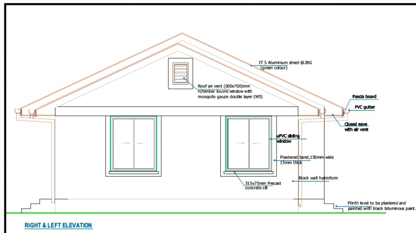
SIDE ELEVATION NHC Mwongozo Housing Estate
